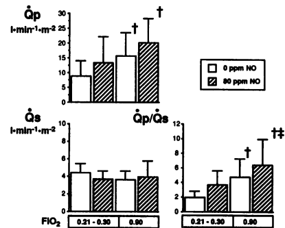
FIGURE 2. Bar graphs of hemodynamic effects of breathing at FiO 2 0.9 and 80 ppm NO by six pediatric patients with congenital heart disease and an intracardiac shunt. Units for blood flow (Q̇) are l·min -1 ·m -2 . †p<0.05 value differs from FiO 2 0.21 without NO. ‡p<0.05 value differs from FiO 2 0.21 with 80 ppm NO. Breathing 80 ppm NO at FiO 2 0.9 increased pulmonary blood flow (Q̇ p ). Inhaling 80 ppm NO at FiO 2 0.21–0.3 and 0.9 did not alter systemic blood flow (Q̇ s ). Breathing at FiO 2 0.9 with or without 80 ppm NO increased Q̇ p /Q̇ s . Maximum elevation of Q̇ p /Q̇ s occurred while inhaling 80 ppm NO at FiO 2 0.9.
