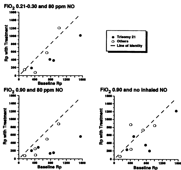
FIGURE 3. Scatterplots of hemodynamic effects of breathing at FiO_2 0.90 and 80 ppm NO by 10 pediatric patients with congenital heart disease and pulmonary artery hypertension. The units of pulmonary vascular resistance index ( R_p ) are \text{dyne} \cdot \text{sec} \cdot \text{cm}^{-5} \cdot \text{m}^{-2} . The baseline R_p was measured while breathing at FiO_2 0.21–0.30 without addition of NO gas. The R_p with treatment was during breathing at FiO_2 0.21–0.90 with or without 80 ppm NO. ●, Values from patients with Trisomy 21; ○, values from patients without Trisomy 21. The stippled line is where the treatment would not change pulmonary pressure from baseline values. Inhaling NO at FiO_2 0.21–0.90 reduced R_p in the many patients; those with a higher baseline pulmonary hypertension had greater pulmonary vasodilation. In all patients with Trisomy 21 (●), inhaling 80 ppm NO at FiO_2 0.21–0.90 reduced R_p . Breathing at FiO_2 0.90 without NO did not consistently reduce R_p .
